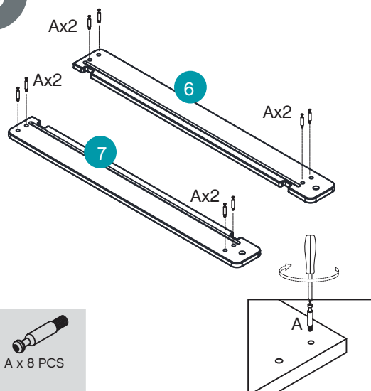
Assemble bolts
