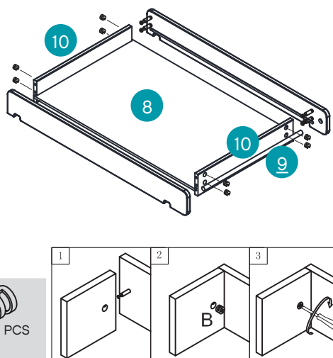
Assemble nuts
